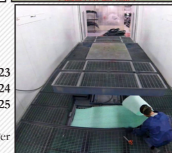
Clean Air Flow Ceiling Filters 560 Grade
