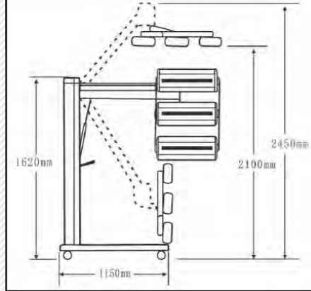
Infrared 3W Short Wave 3 Bar & Infrared 2AT Shortwave High Reach 2 Bar SKU: FY-3W SKU: FY-2AT
