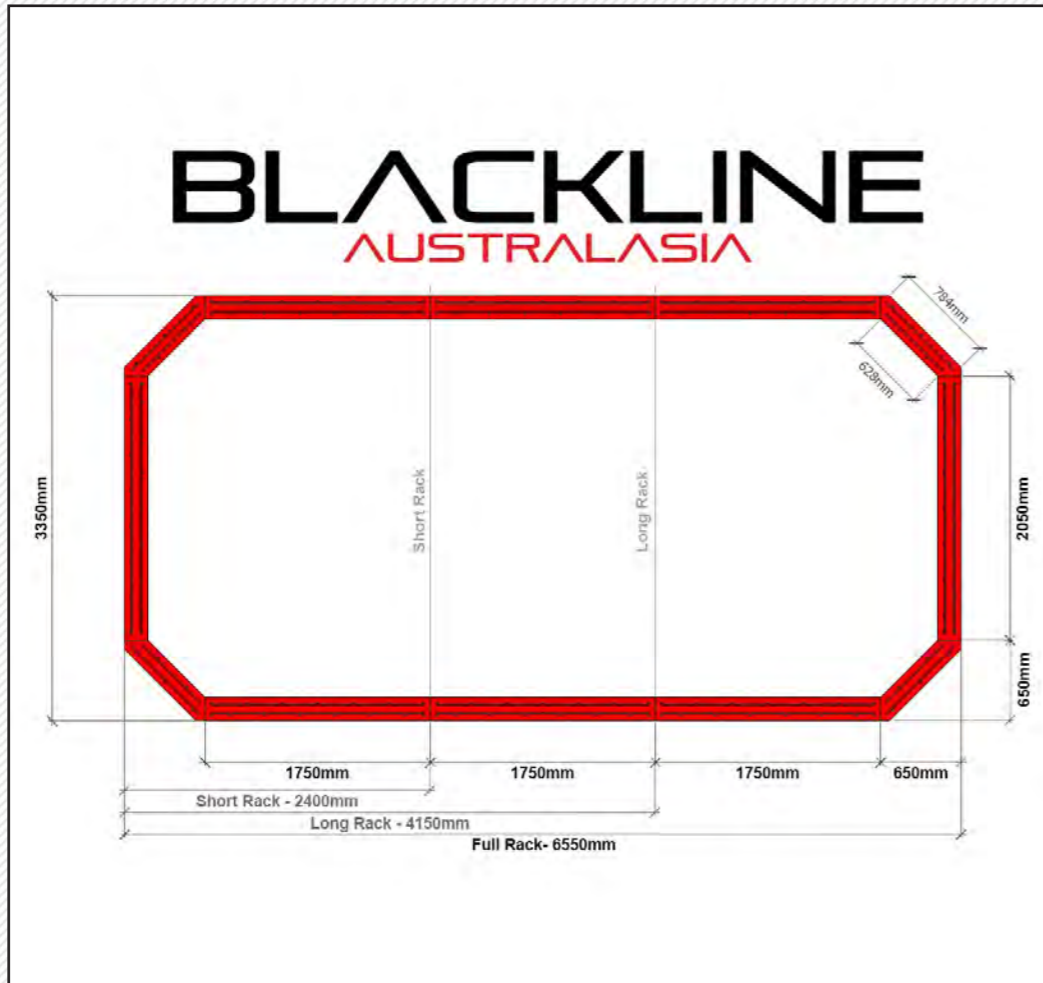
Complete Flat Rack and Pulling Tower SKU: BLPRACK
